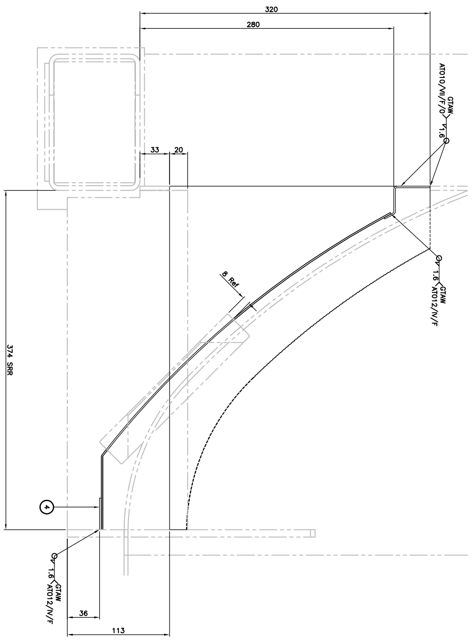
SECTIONAL VIEW - A
